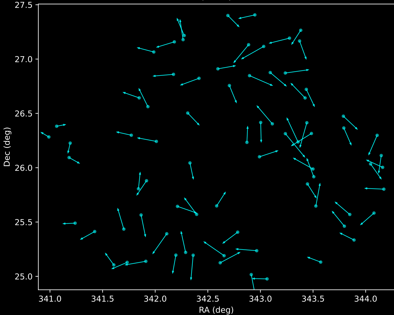
APOGEE DR17 Noise Stream Proper Motion Vectors (n=76)
