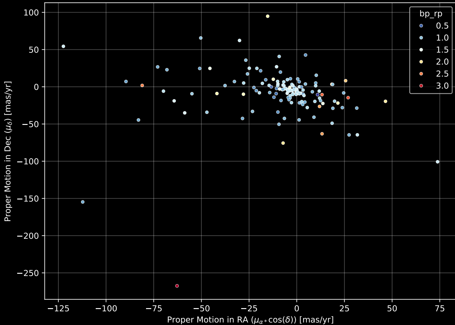
APOGEE DR17 Field: [043+46_MGA] Proper Motion Diagram (n= 140)
