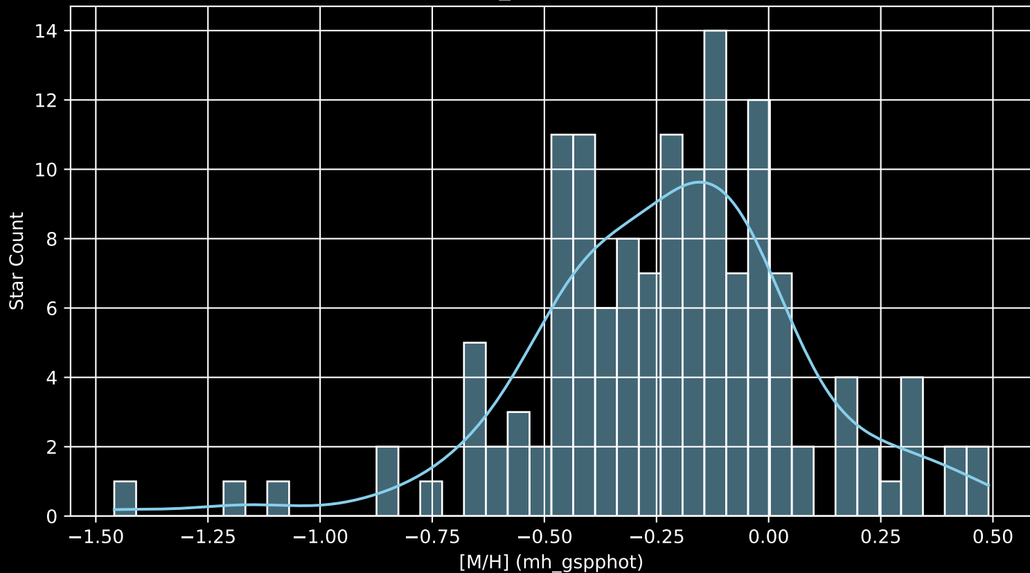
APOGEE DR17 Field: [043+46_MGA [M/H] (mh_gspphot) (n= 139)
