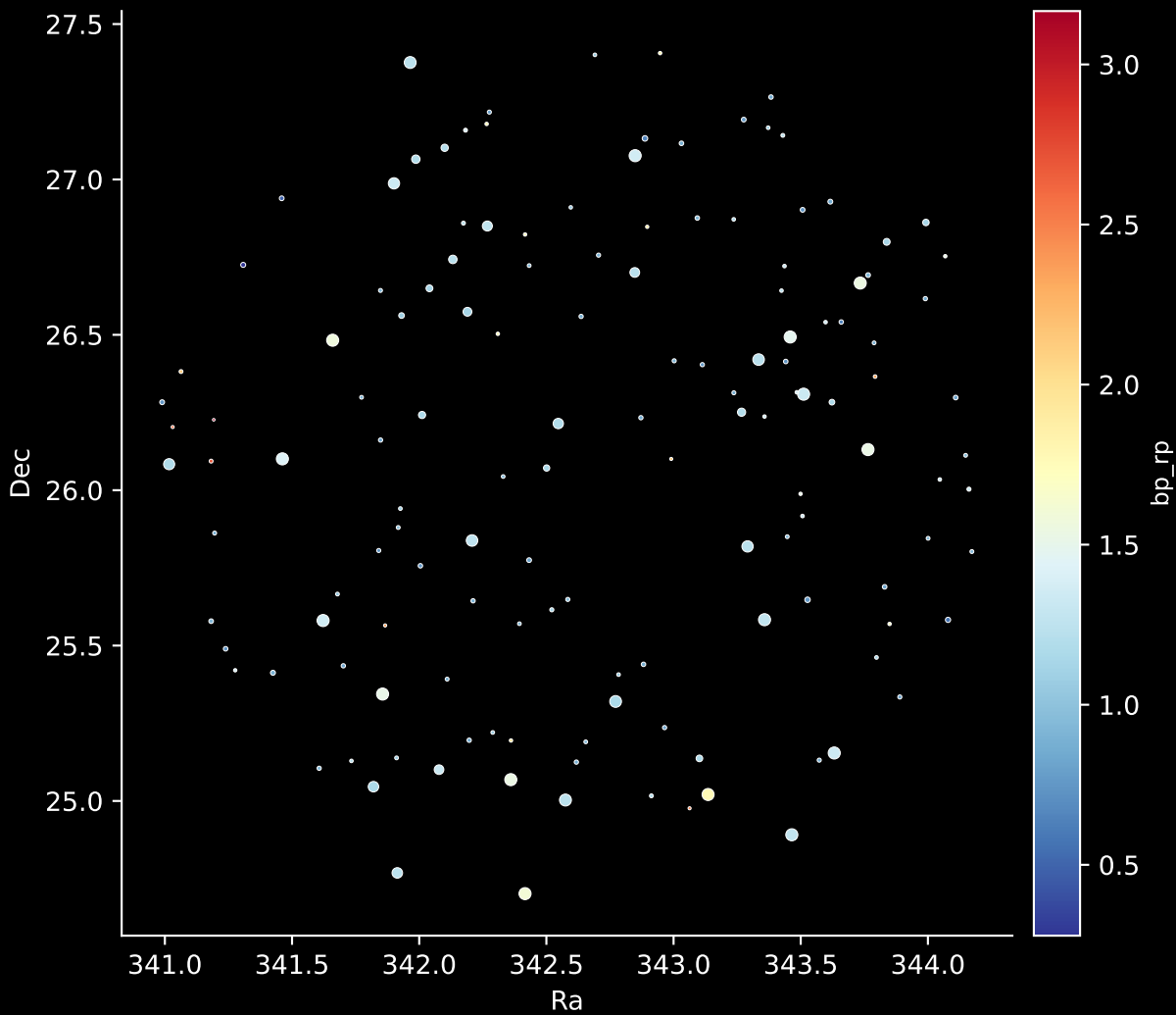
APOGEE DR17 Field: [043+46_MGA] Stars: 140
