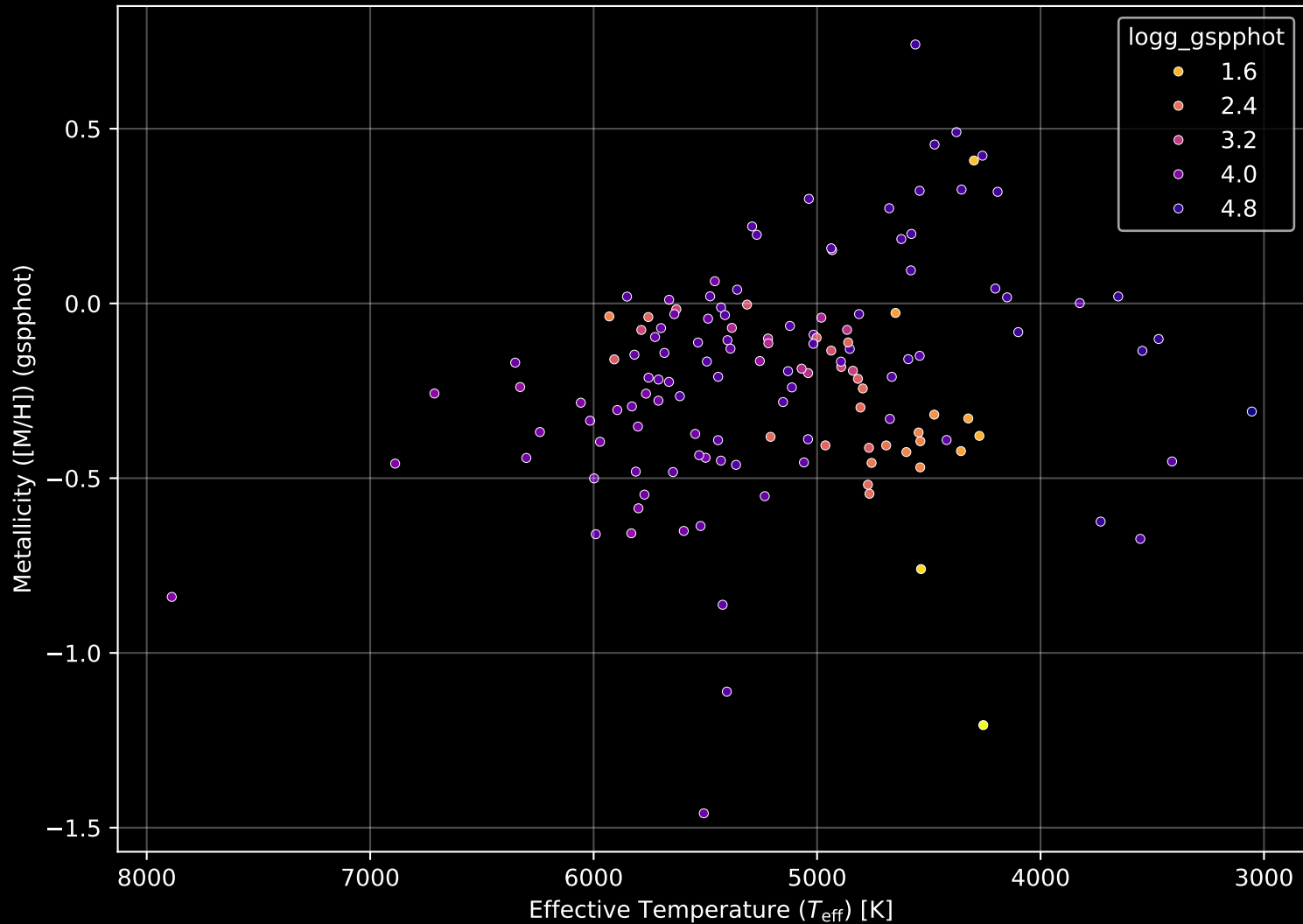
APOGEE DR17 Field: [043+46_MGA] Stellar Population Parameters (n= 140)
