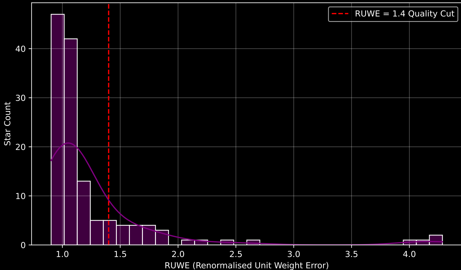
GAPOGEE DR17 Field [043+46_MGA] RUWE Distribution (n= 135)
