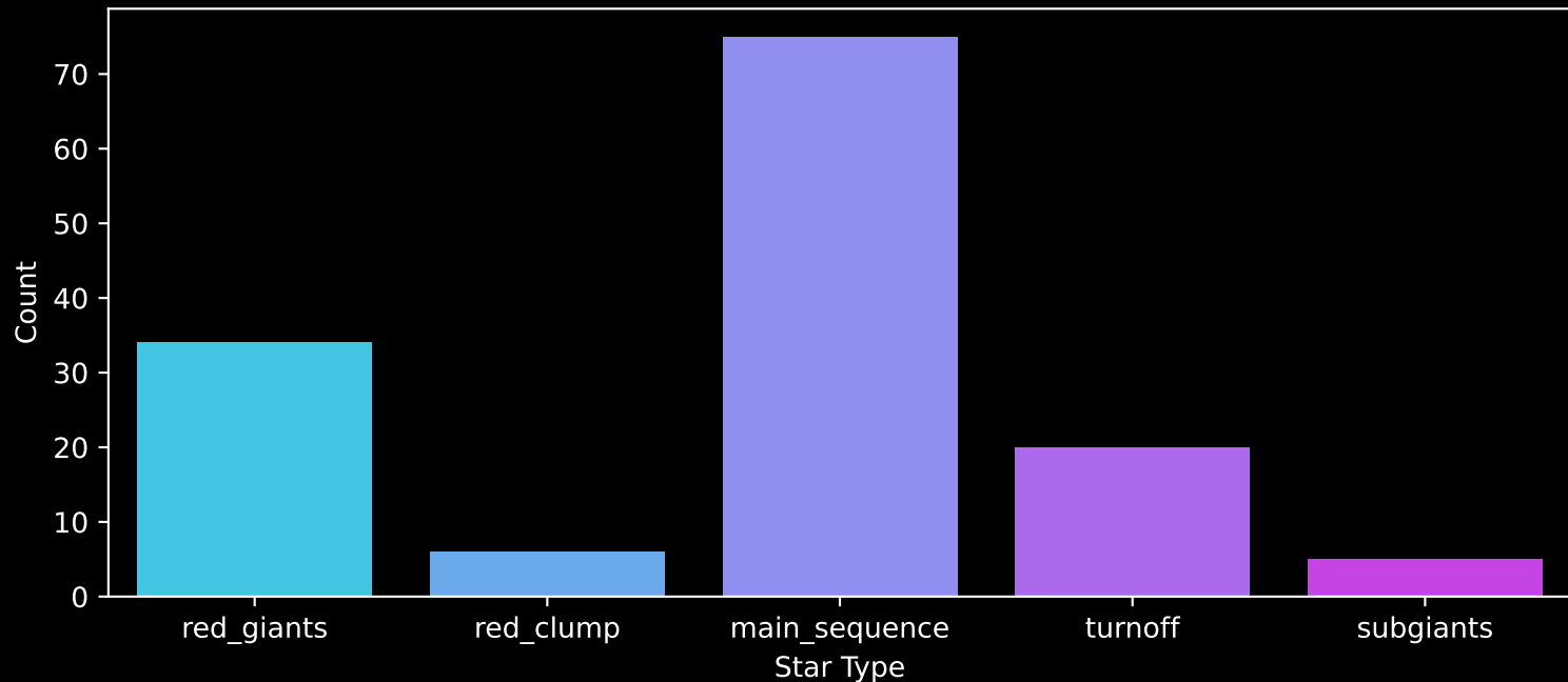
APOGEE DR17 Field: [043+46_MGA] Count plot of Star Type
