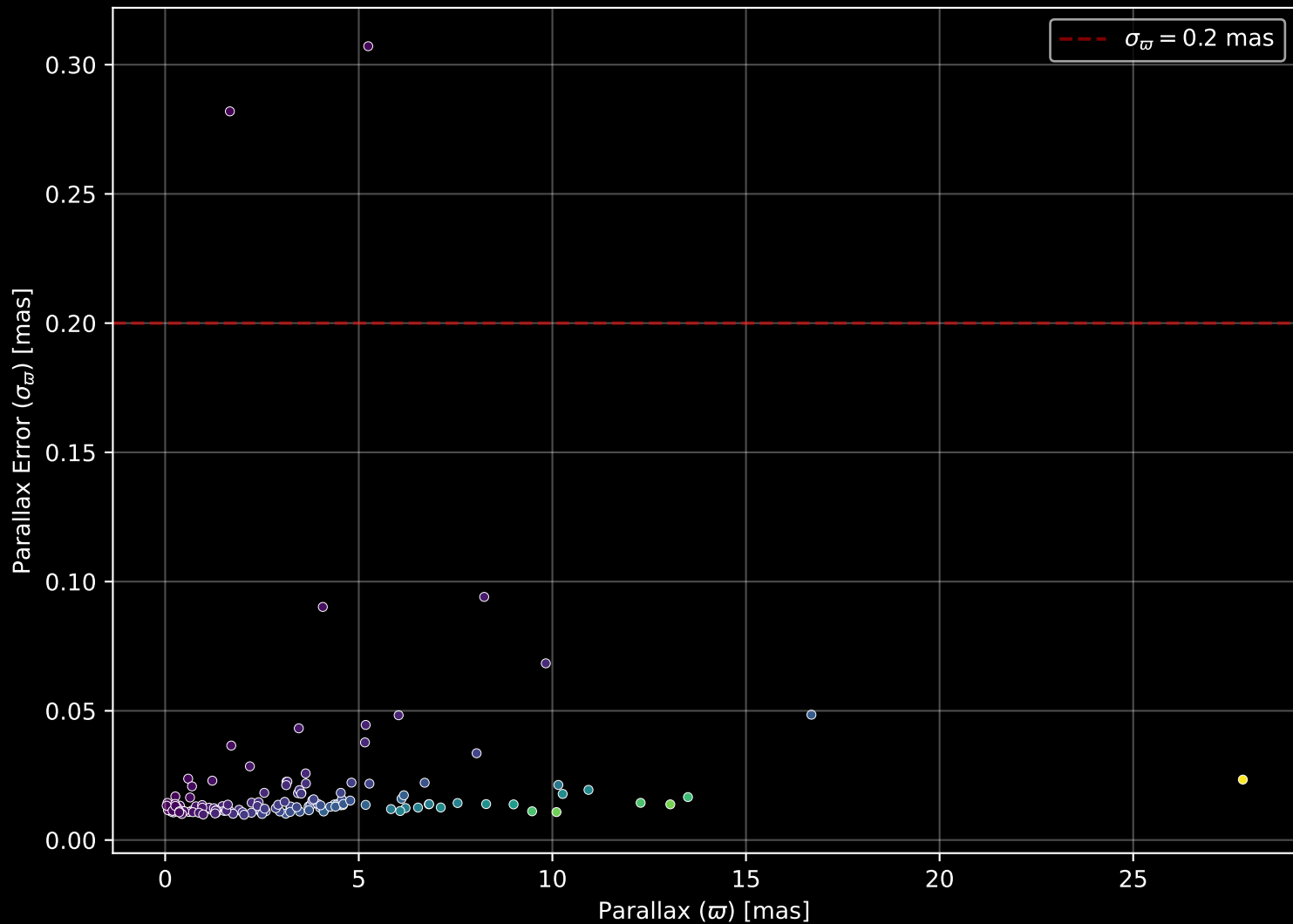
APOGEE DR17 Field: [043+46_MGA] Parallax Quality (n= 140)
